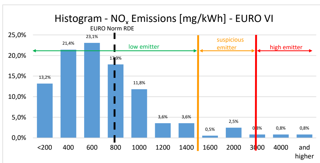
Figure 24: Histogram of observed emissions for EURO VI HDV.
