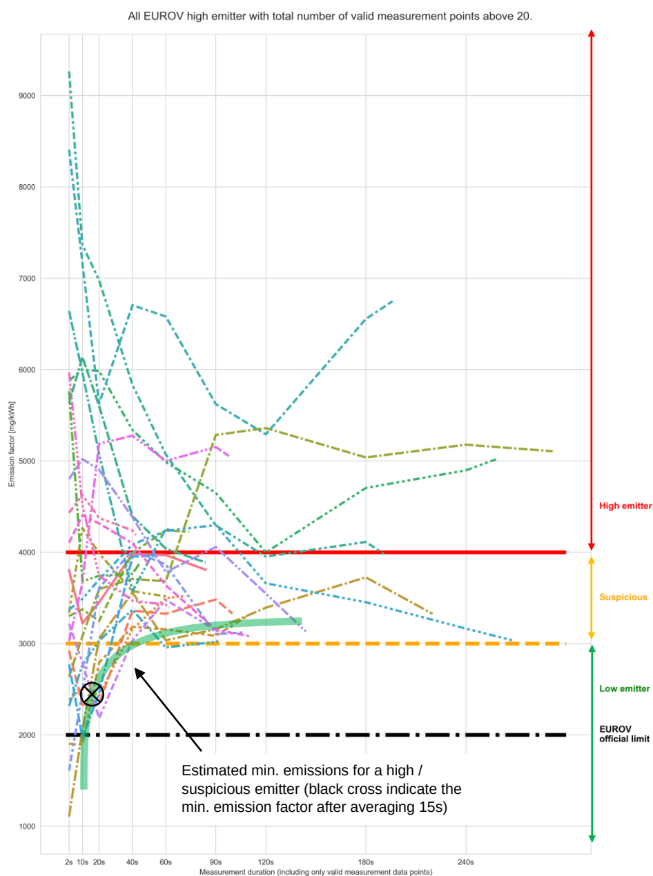
Figure 44: Average NO x emission value for EURO V HDV classified finally as suspicious or high emitters in dependence of the averaging time (x-axis). Each line represents one individual measured HDV. An envelope of the estimated minimum emissions for a high / suspicious emitter are drawn and the cross indicate the recommended estimated limit after 15 seconds (recommended time for preliminary emission value).
