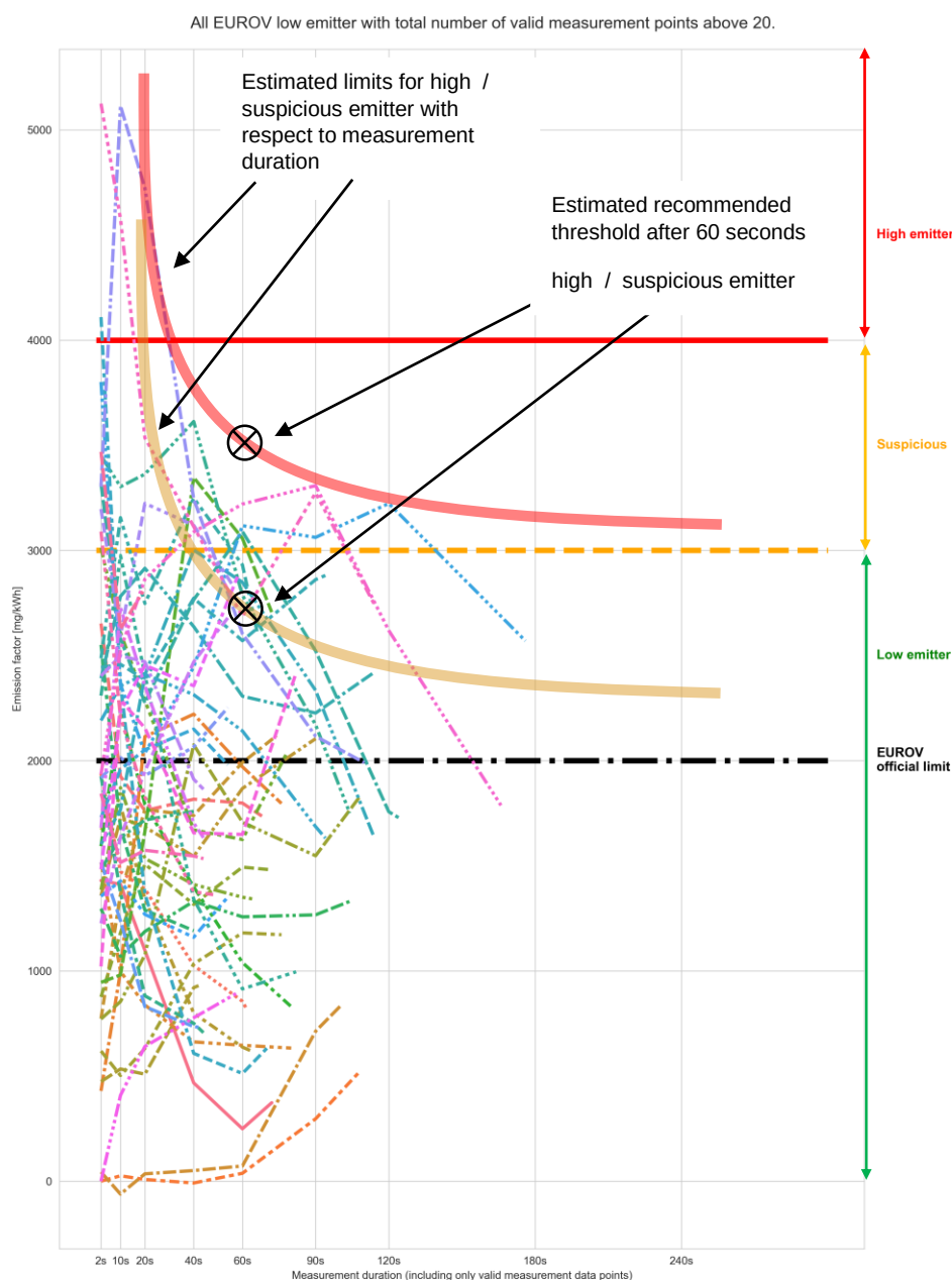
Figure 43: Average \text{NO}_x emission value for EURO V HDV classified finally as low emitters in dependence of the averaging time (x-axis). Each line represents one individual measured HDV. An envelope of the estimated maximum emissions for a high / suspicious emitter are drawn and the cross indicate the recommended limit after a measurement period of 60 seconds.
