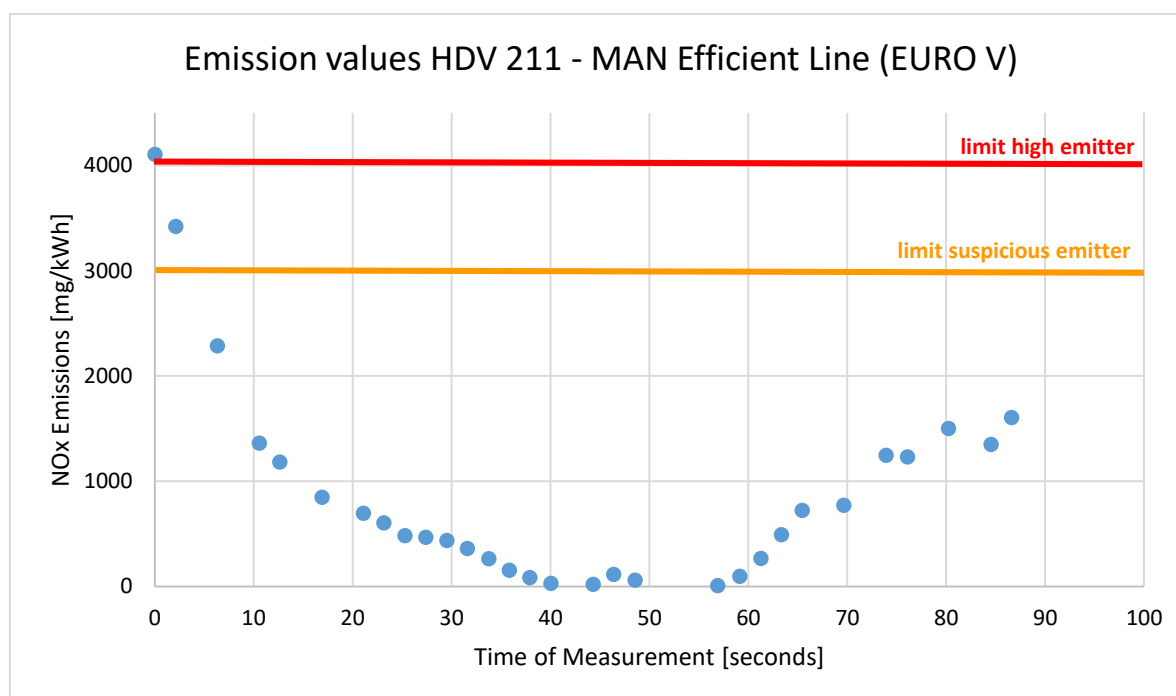
Figure 35: Time series of NO x emission factor for measured HDV no 211 (EURO V) with SCR warm-up. Each data point represents the instantaneous emission value, not the averaged emission over time. The limit indicates the used limits for the average emission value in this study to identify a suspicious and high emitter.
