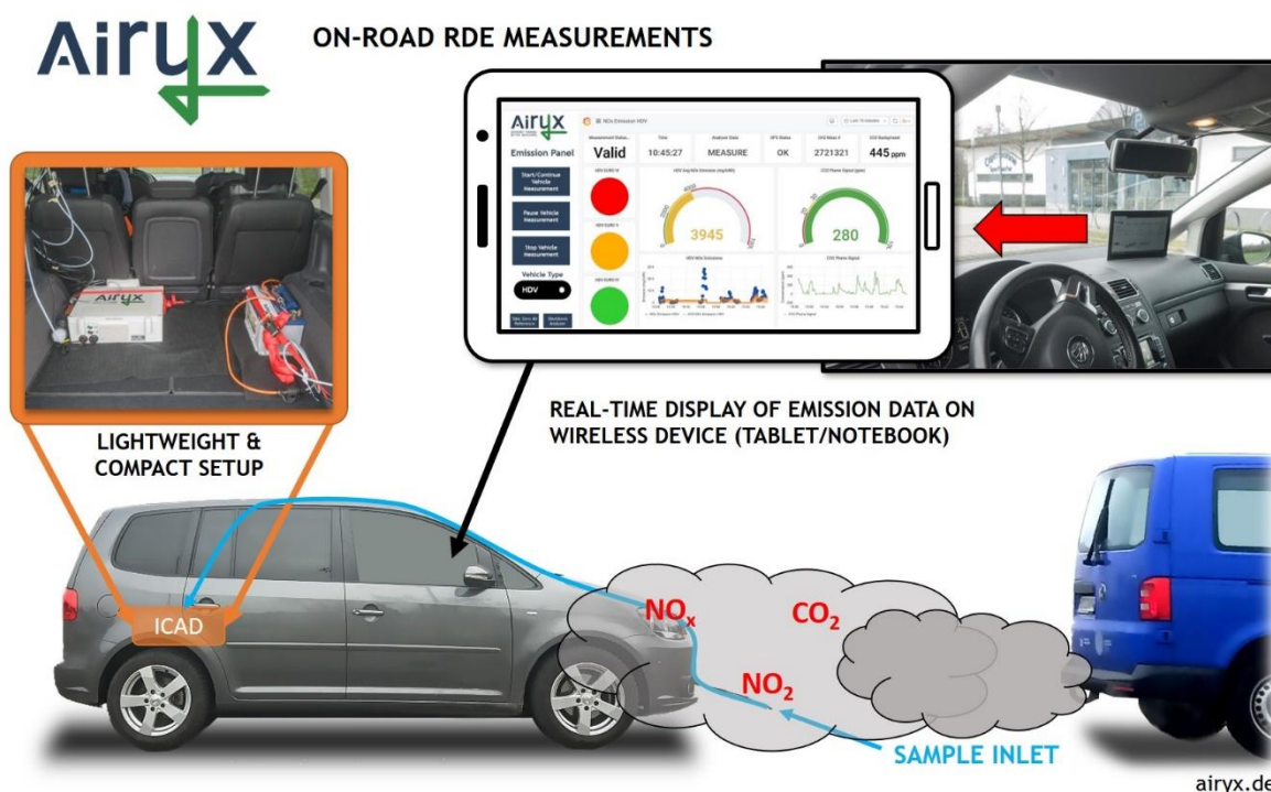
Figure 1: Basic sketch of plume chasing measurement principle from Airyx GmbH. The diluted exhaust gases are sampled and analysed. Different gases are measured with the ICAD instrument. From the ratio of the gases, emission factors of the followed vehicle are derived.
