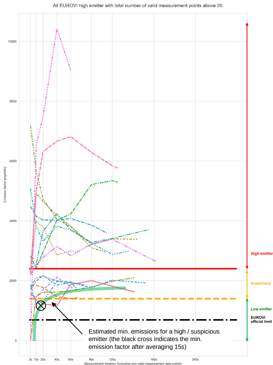
Figure 42: Average \text{NO}_x emission value for EURO VI HDV classified as suspicious or high emitters in dependence of the averaging time (x-axis). Each line represents one individual measured HDV. An envelope of the estimated minimum emissions for a high / suspicious emitter are drawn and the cross indicate the recommended estimated limit after 15 seconds (recommended time for preliminary emission value).
